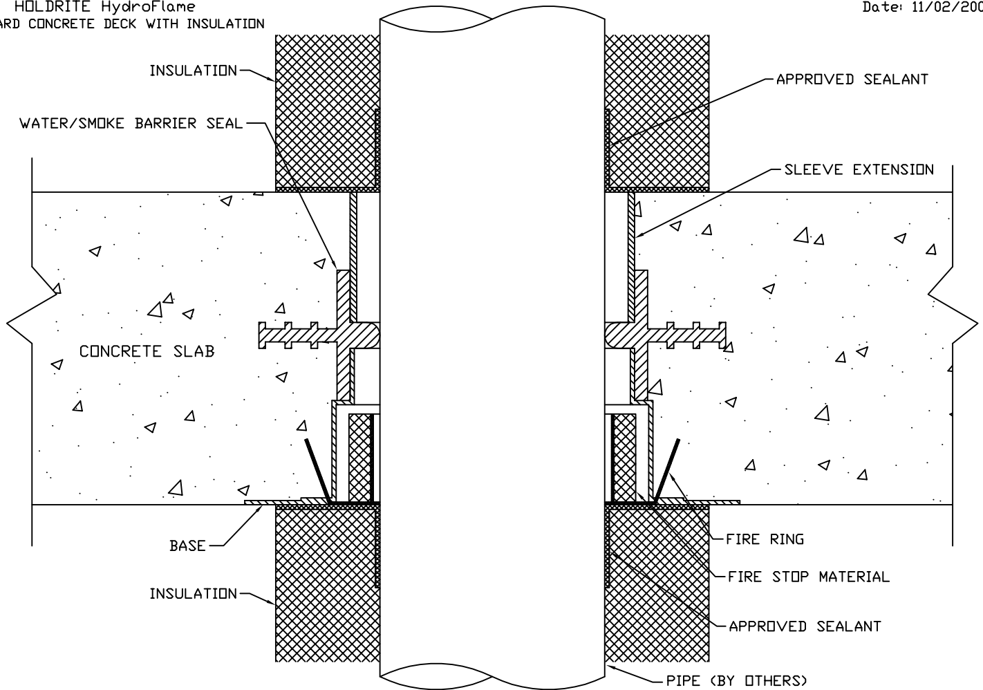
(11) Floor, Water/Air/Smoke Tight Sleeve, Metallic Pipe w/Insulation, B&W Detail
