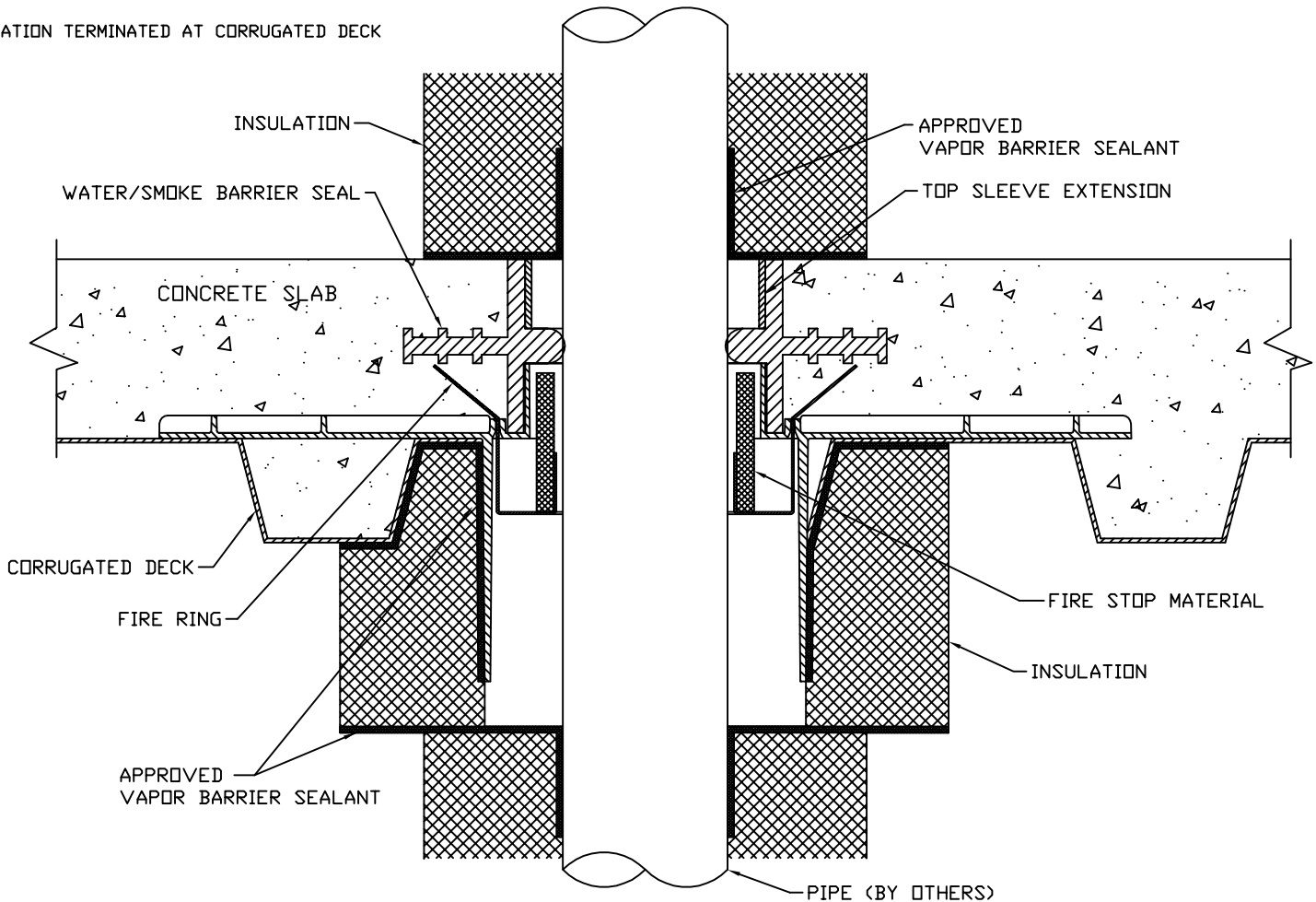
(15) Corrugated Floor, Water/Air/Smoke Tight Sleeve, B&W Detail
